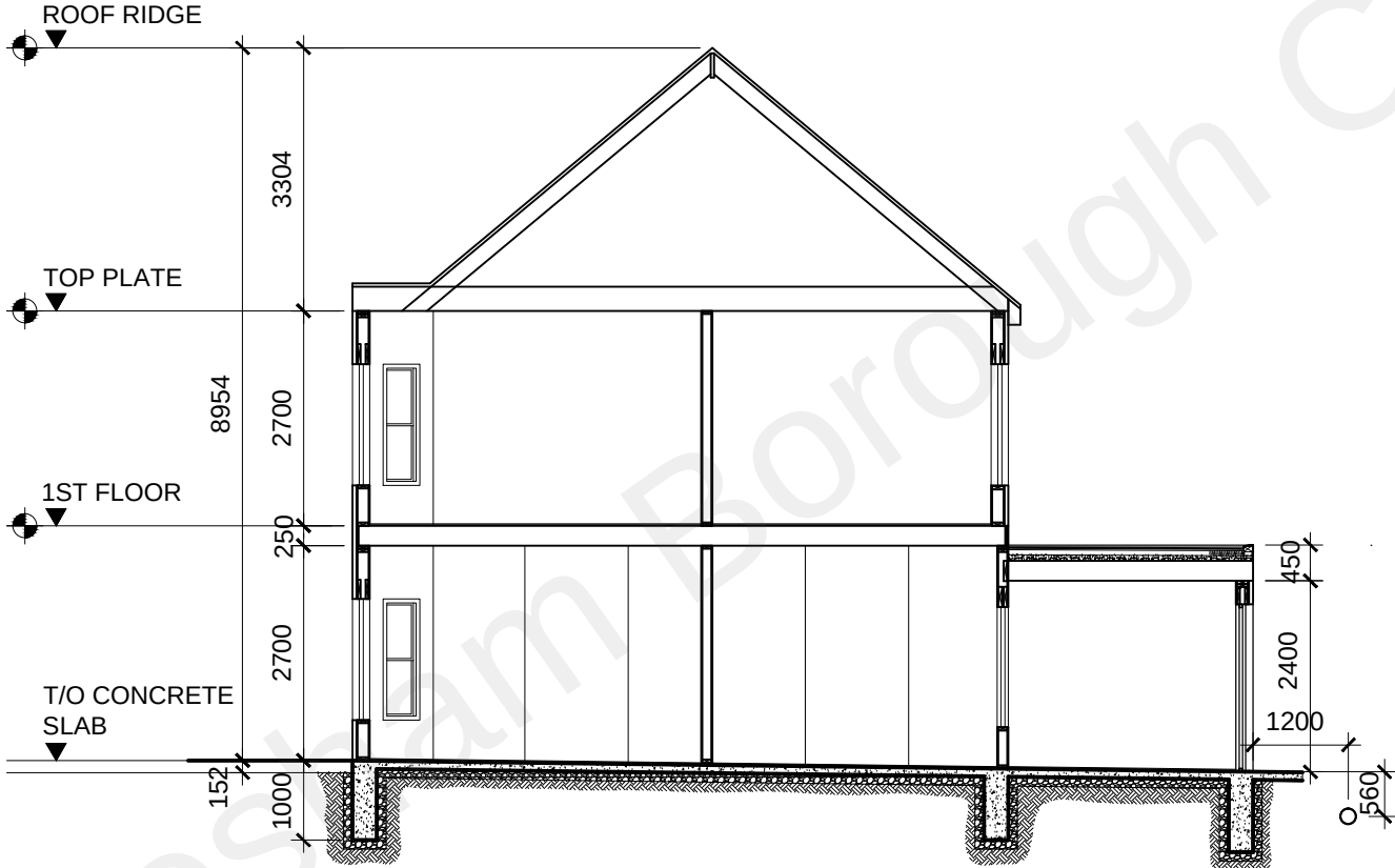
SECTION - A ( PROPOSED )
