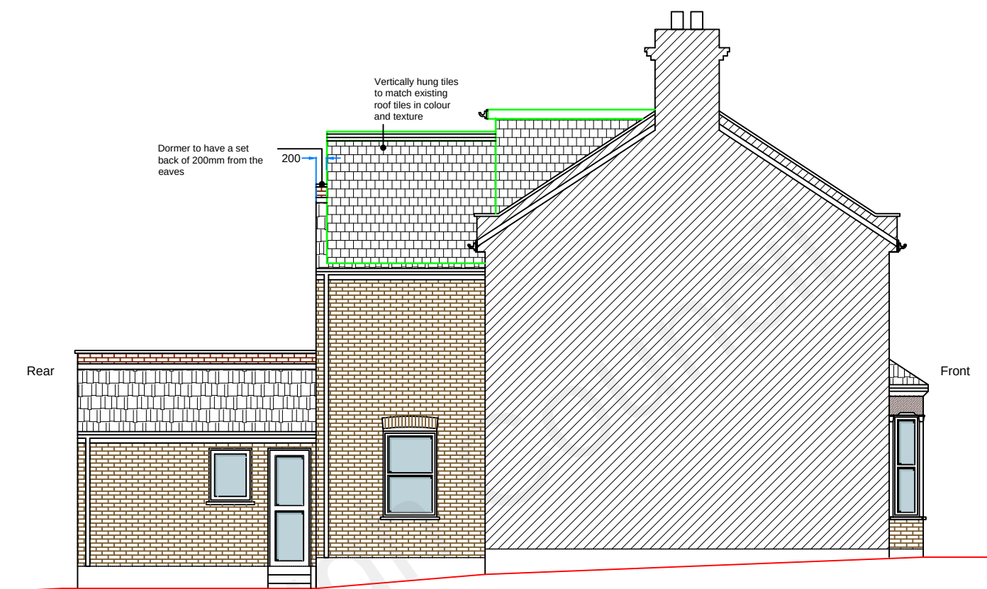
PROPOSED FLANK ELEVATION
