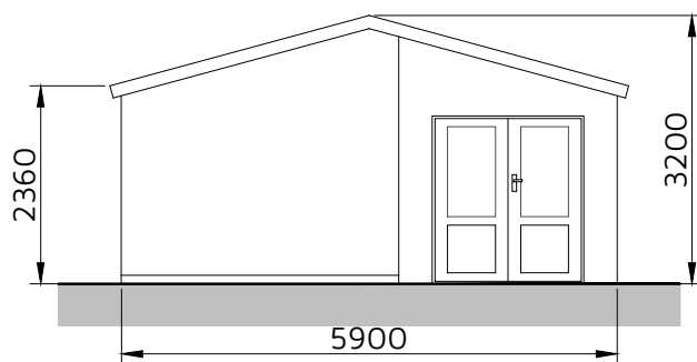
1. Proposed Side Elevation 1:100 @ A4
