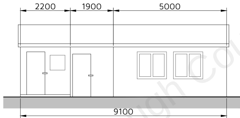
2. Proposed Front Elevation 1:100 @ A4
