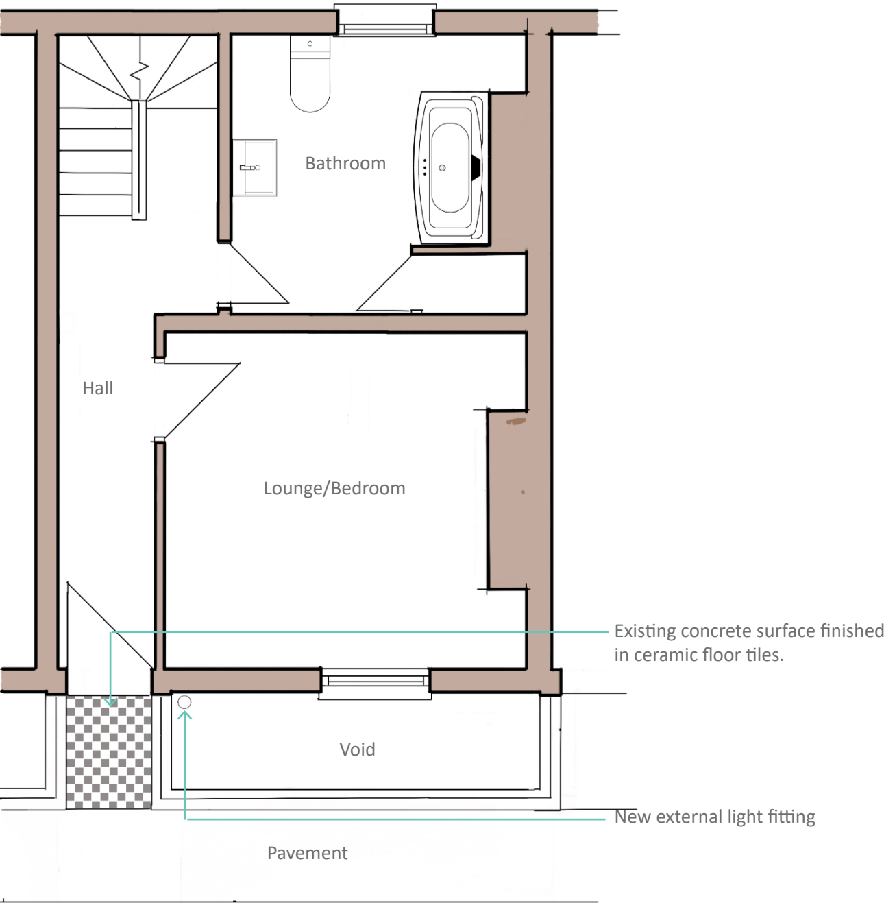
First Floor
