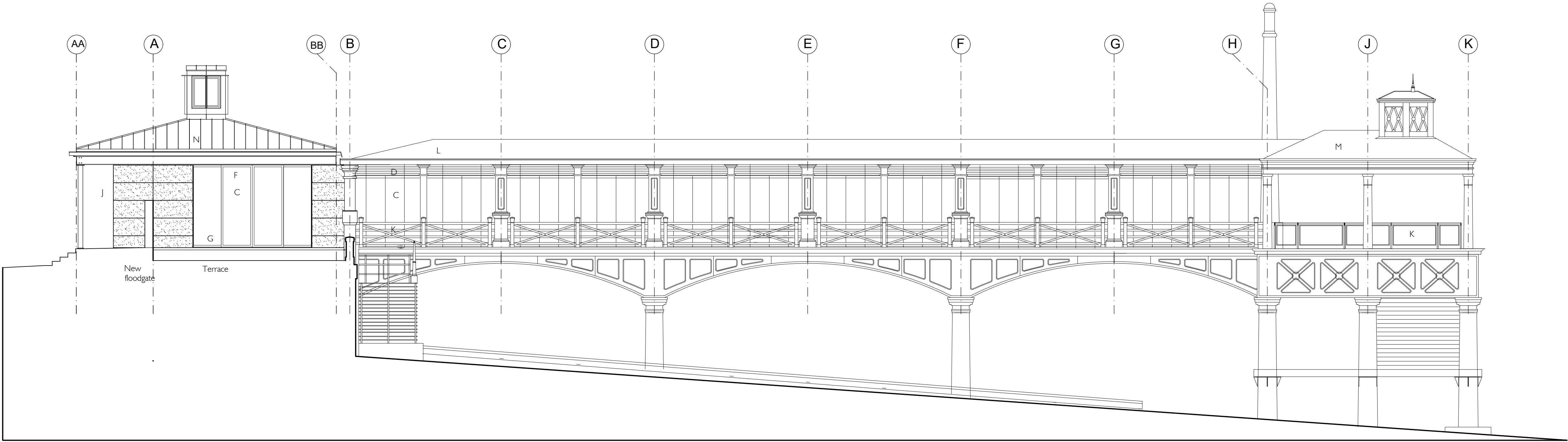
EAST FACING ELEVATION
