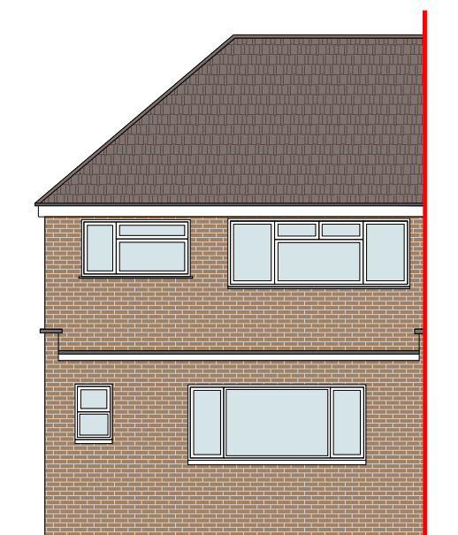
Existing Rear Elevation (North-East)
