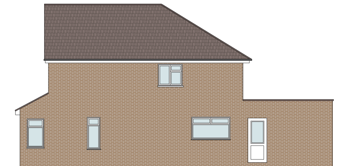
Existing Side Elevation (South-East)
