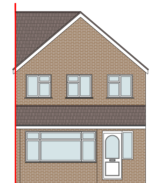
Existing Front Elevation (South-West)
