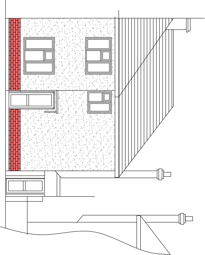
Front Elevation
