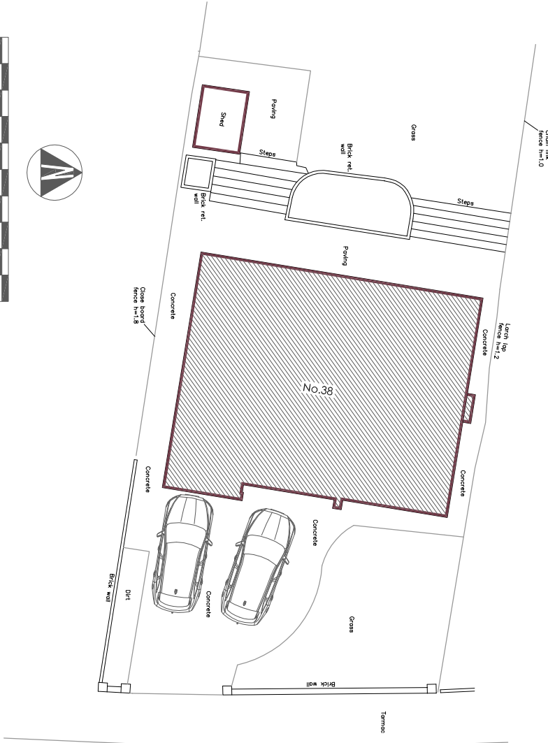
EXISTING SITE PLAN 1:200
