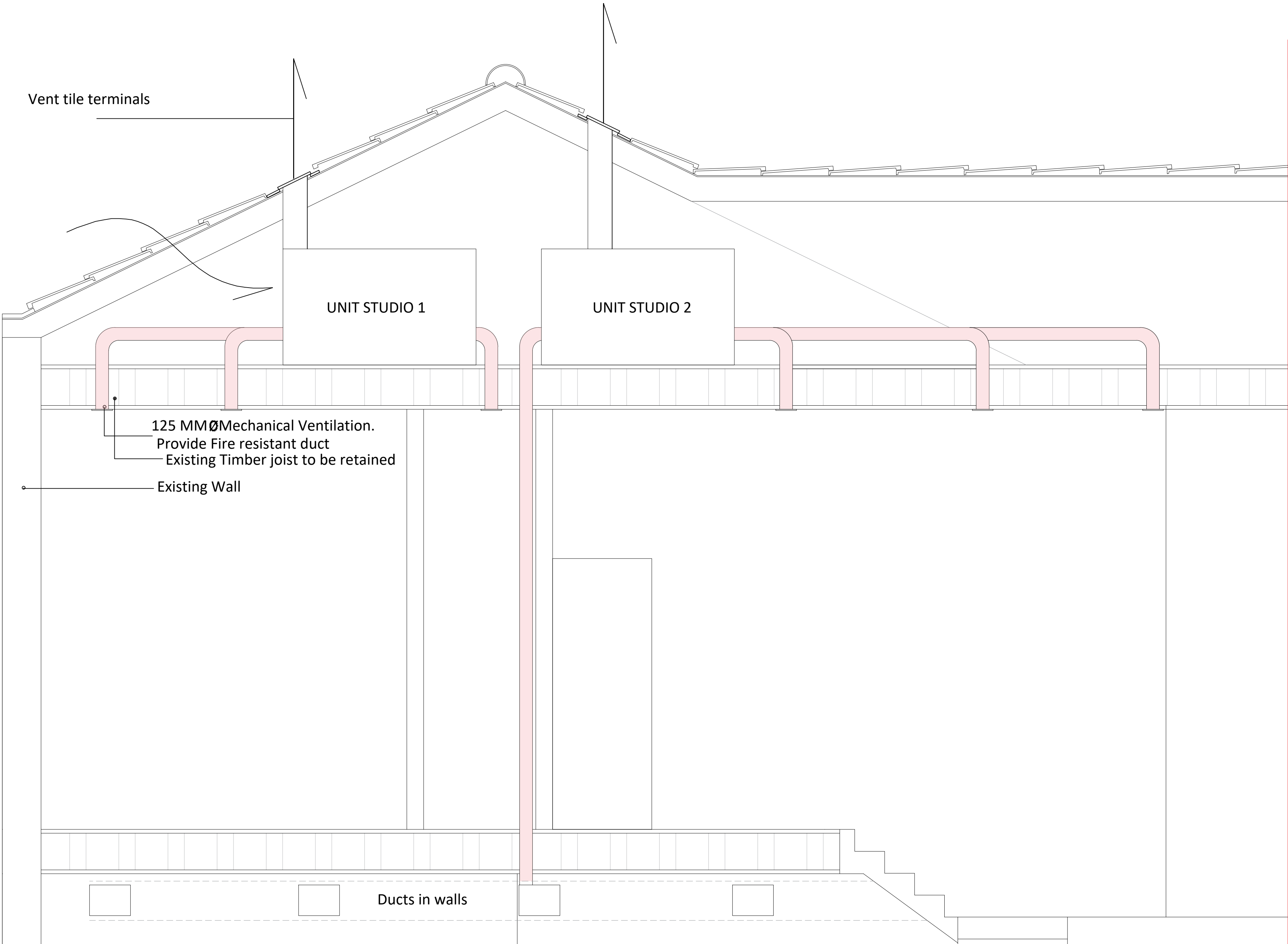
MVHR detail
