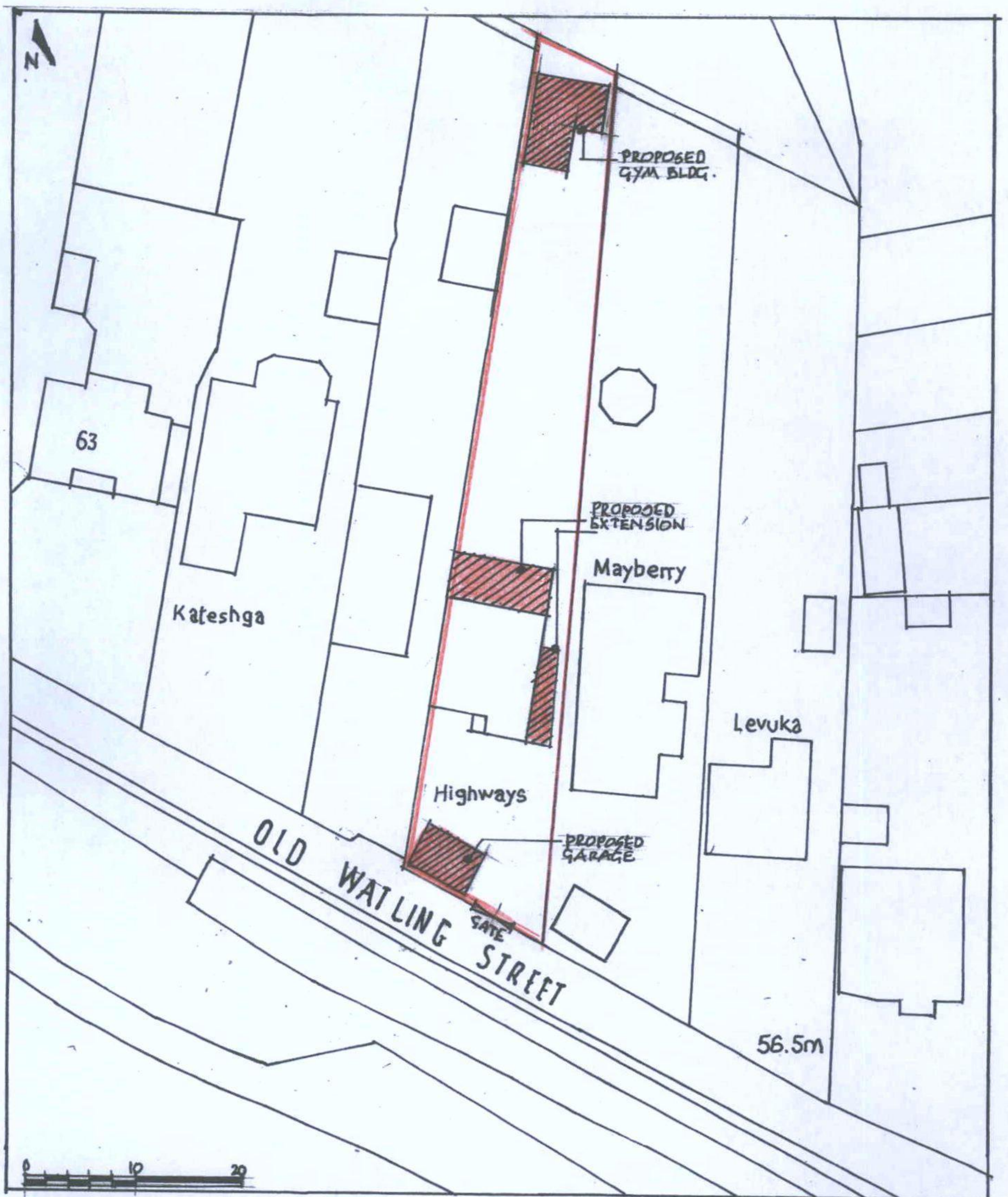
BLOCK PLAN 1:500
