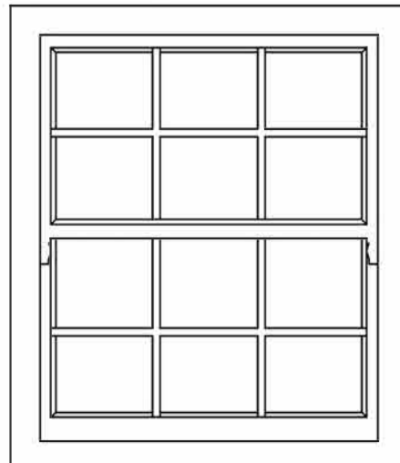
Proposed W17 Left Hand Side Elevation 1:20 @ A3
