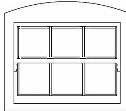
Proposed W14 Right Hand Side Elevation 1:20 @ A3
