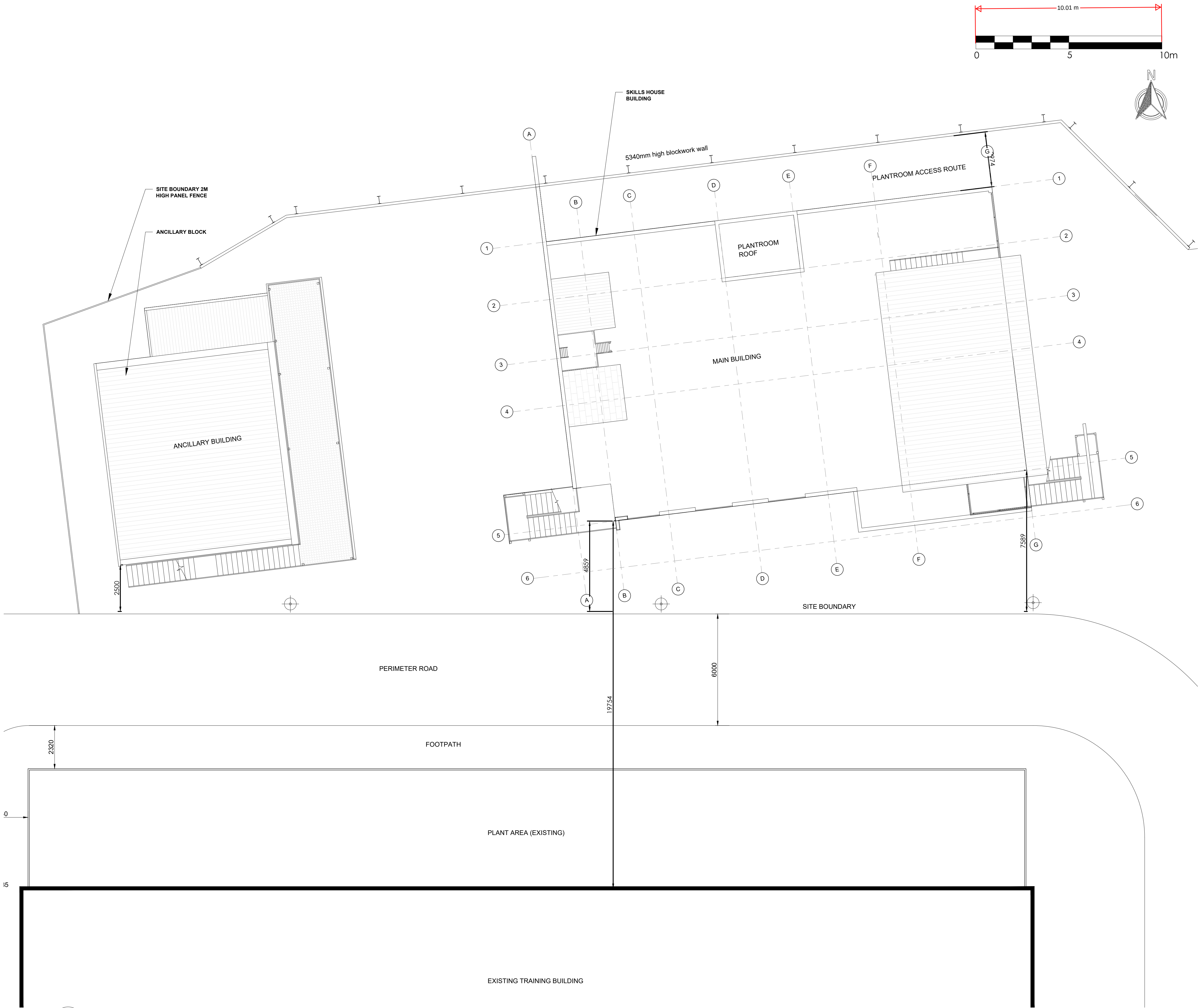
1 EXISTING BLOCK PLAN 101 SCALE 1:100
