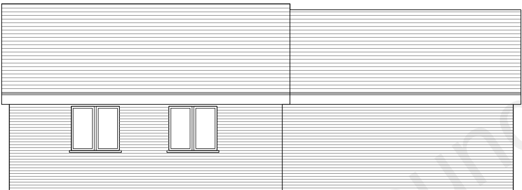
Existing East Elevation 1:100
