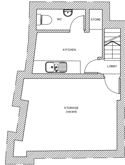
EXISTING BASEMENT FLOOR PLAN 1:100
