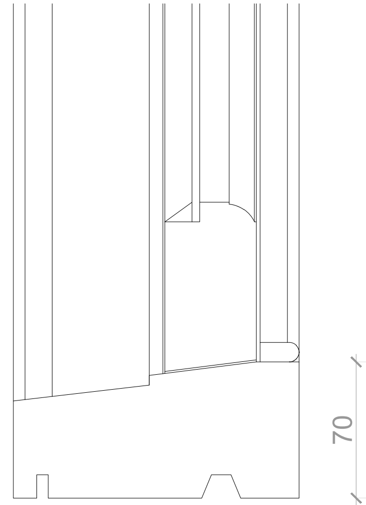
DETAIL 3 Window Cill
