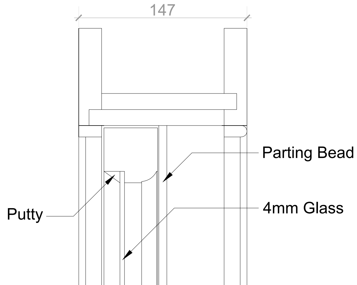
DETAIL 1 Window Head
