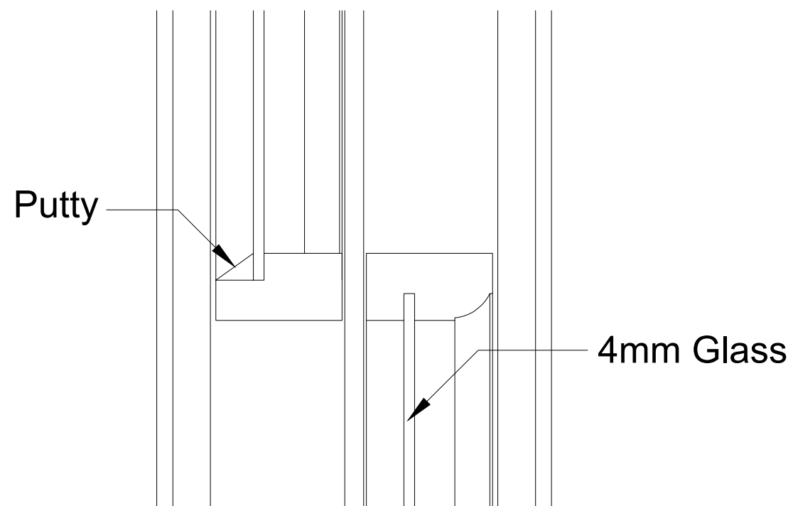
DETAIL 2 Meeting Rail
