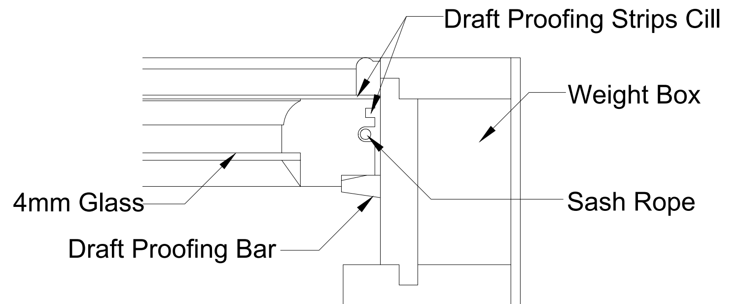
DETAIL 4 Plan through sash box and window
