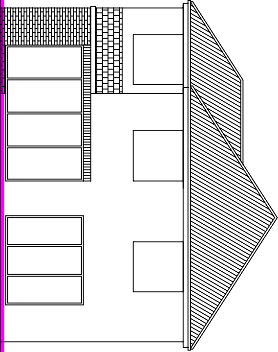
Proposed Elevation
