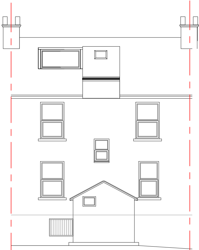
REAR ELEVATION
