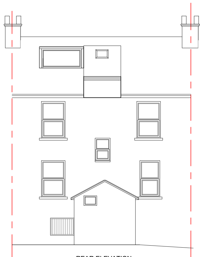
REAR ELEVATION
