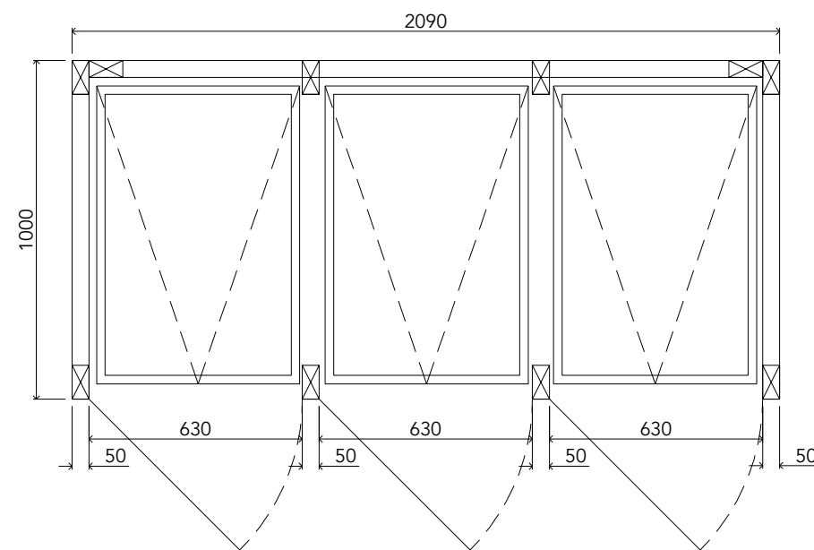
02 | 1:20 | INTERNAL LAYOUT
