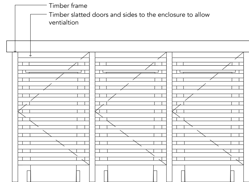
03 | 1:20 | FRONT ELEVATION
