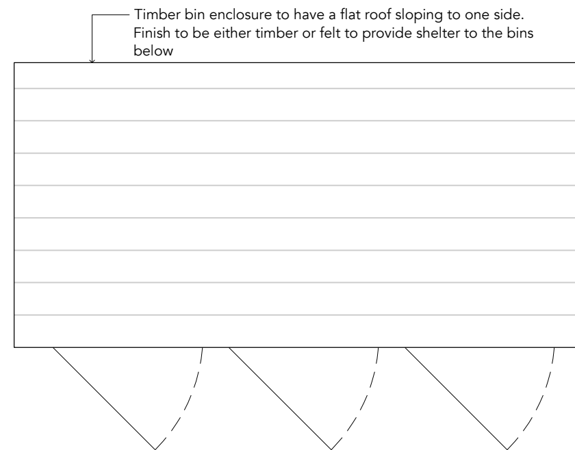
01 | 1:20 | BIN STORE ROOF PLAN
