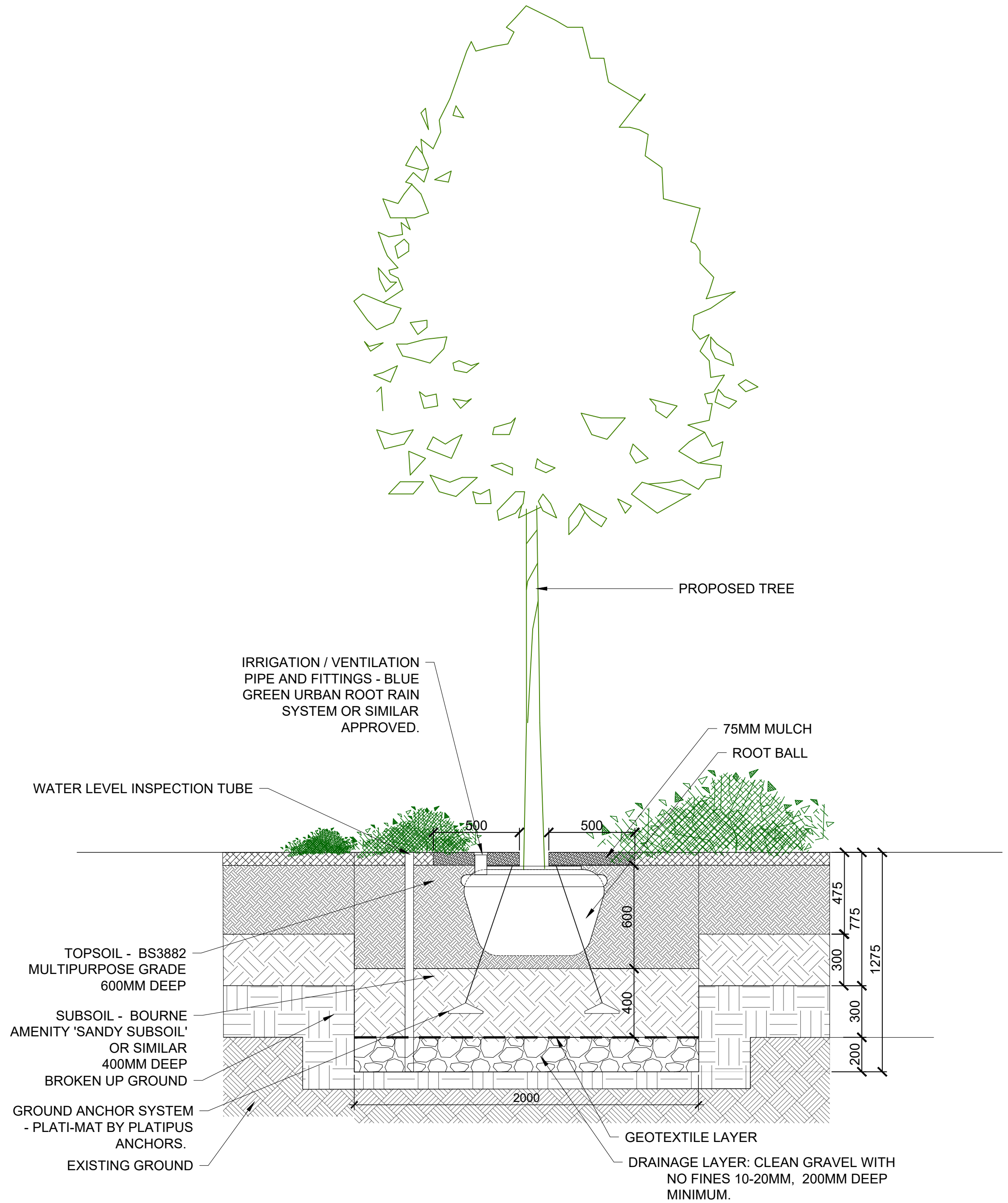
3 Section: Tree Pit in Soft Landscape 1:20
