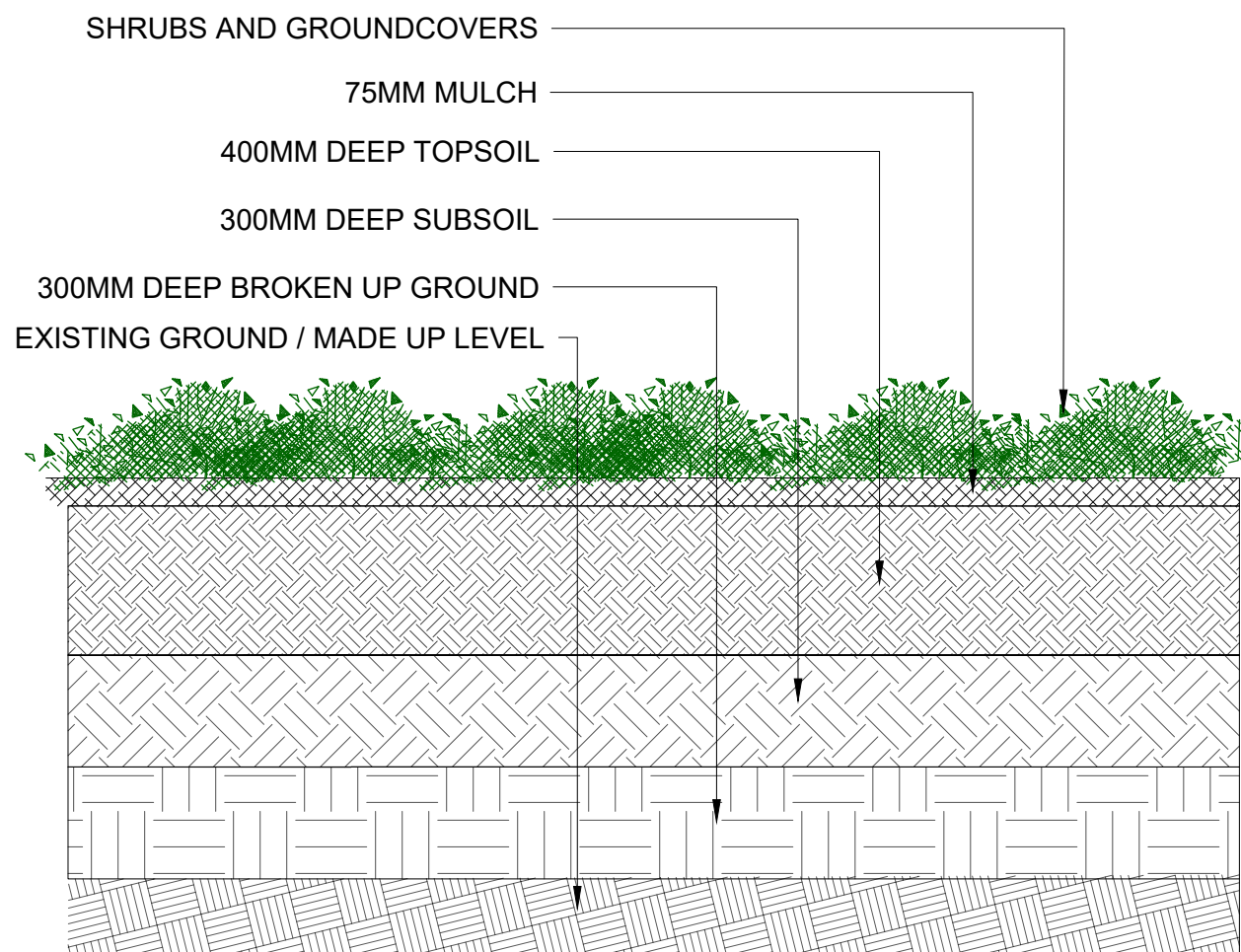
2 Section: Shrub Planting 1:20
