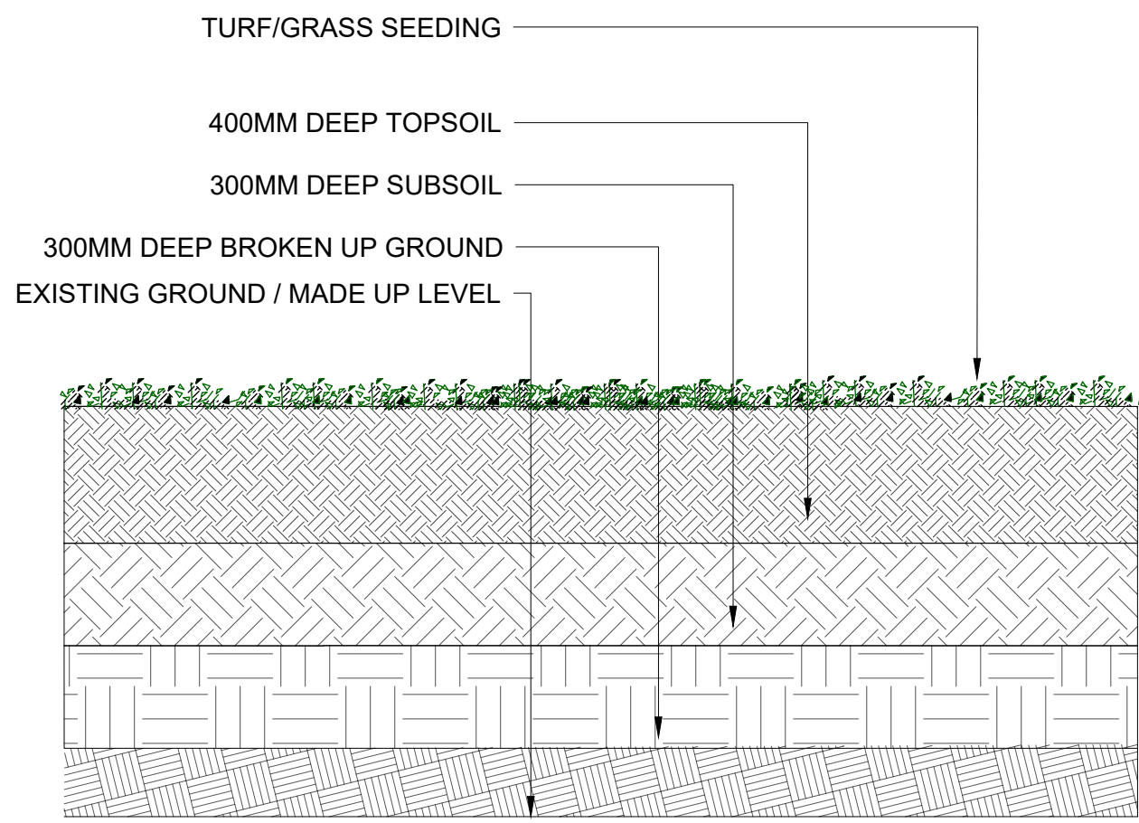
1 Section: Grass/Turf Planting 1:20
