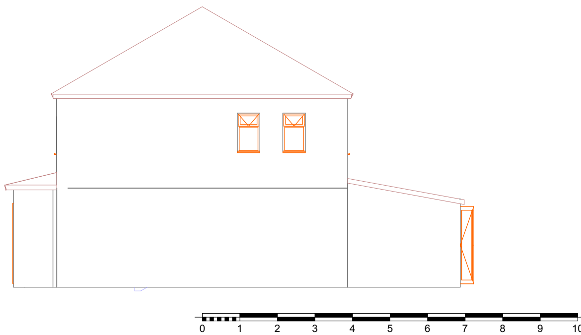
8 Right Elevation Proposed 1:100
