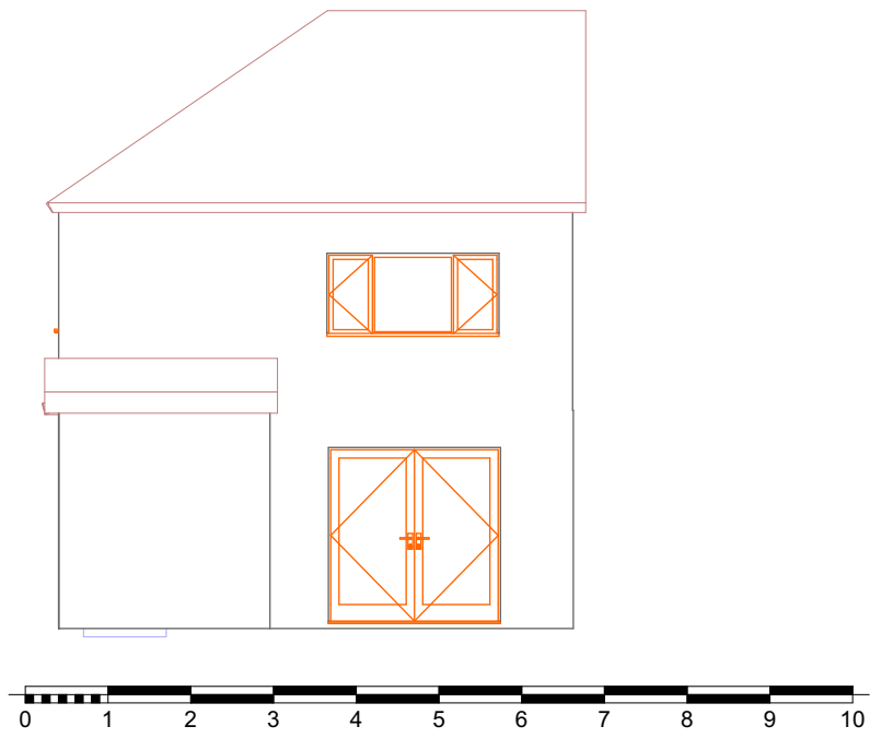
3 Rear Elevation Existing 1:100
