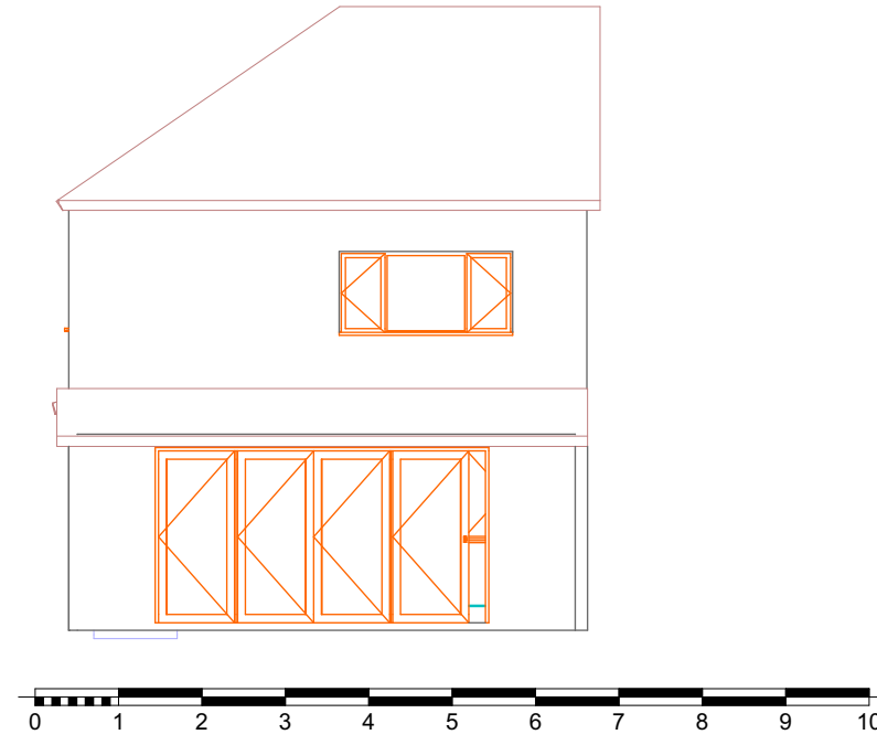
4 Rear Elevation Proposed 1:100
