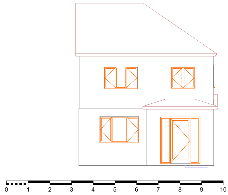
1 Front Elevation Existing 1:100
