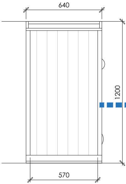
Bin Store - Elevations 3 x 240lt for Non-Recyclable Waste / Recycling / Food Waste
