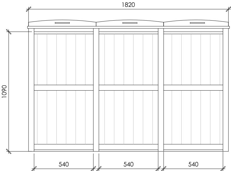
Bin Store - Elevations 3 x 240lt for Non-Recyclable Waste / Recycling / Food Waste
