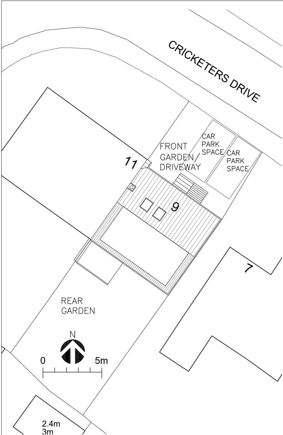
03 PROPOSED BLOCK PLAN SCALE 1:200 @ A3
