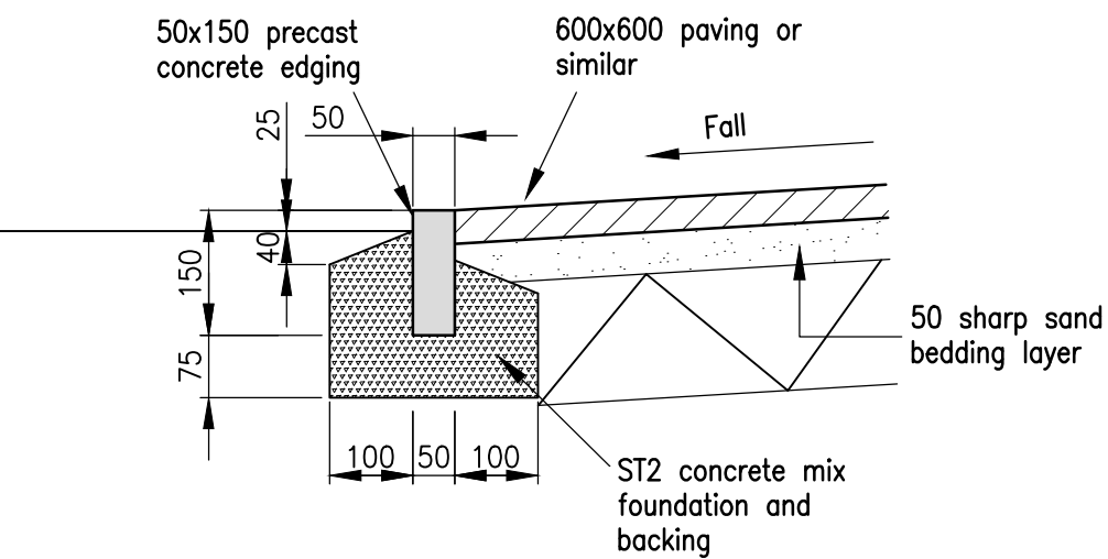
Precast Concrete Kerb Detail Scale 1:10
