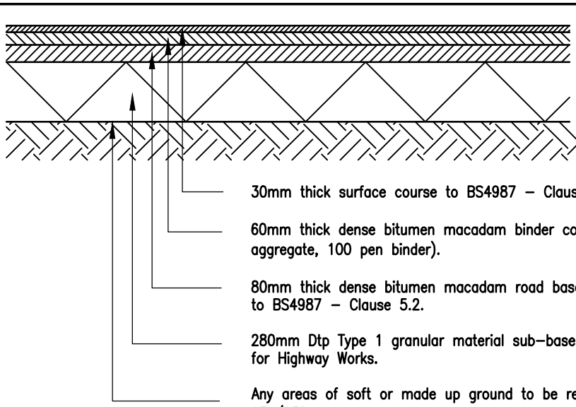
Road Construction Detail Scale 1:20
