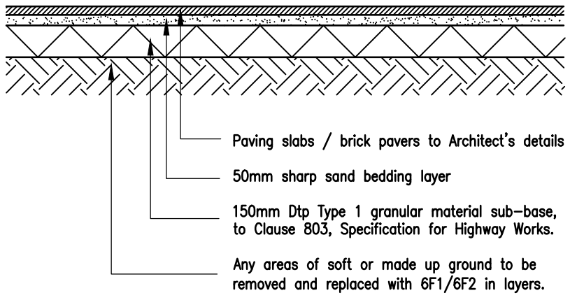
Paving / Brick Pavers Construction Detail Scale 1:20
