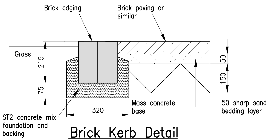
Brick Kerb Detail Scale 1:10
