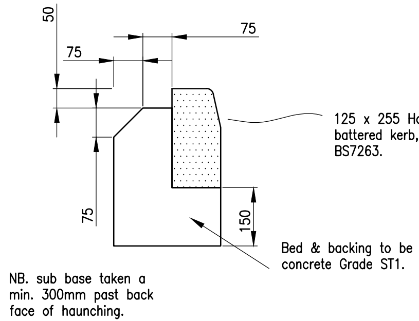
Typical Kerb Detail – Type HB2.
