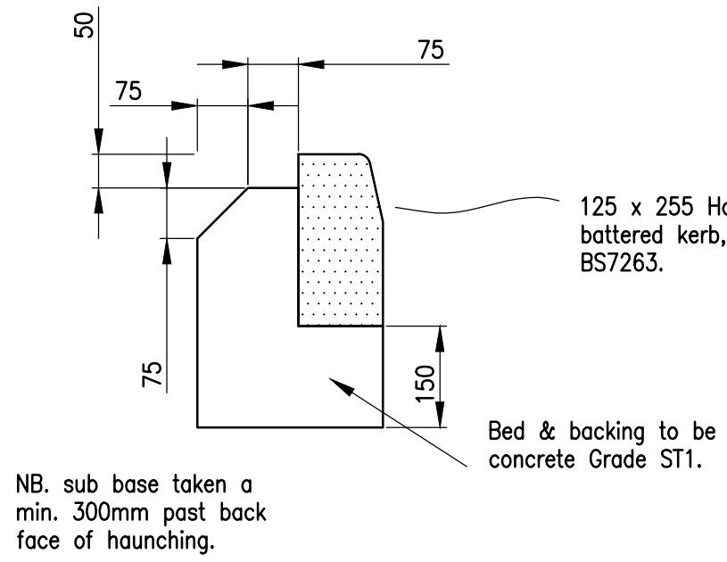
Typical Kerb Detail – Type HB2.
