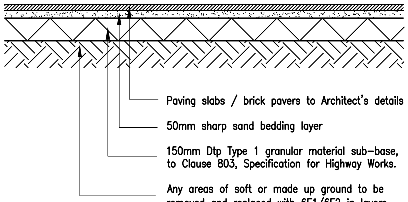
Paving / Brick Pavers Construction Detail Scale 1:25
