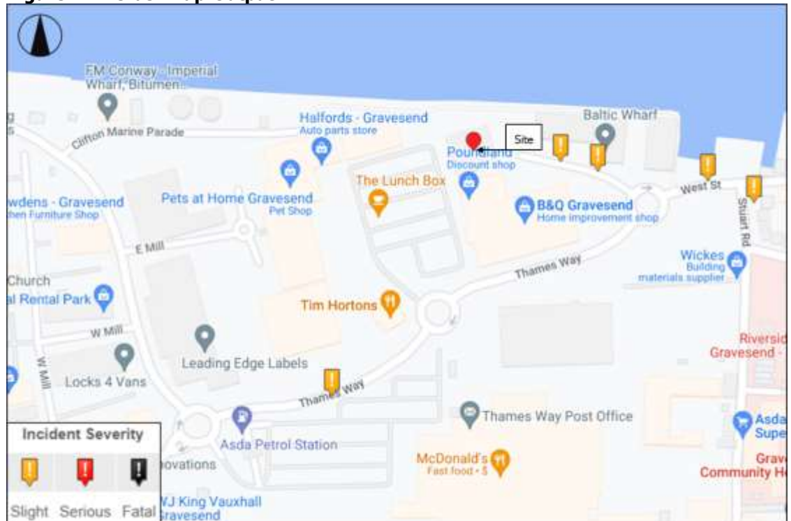
Figure 2.4: CrashMap Output
