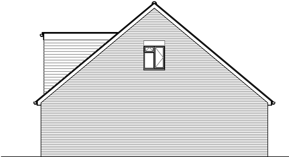
1 Side Elevation Scale 1/100
