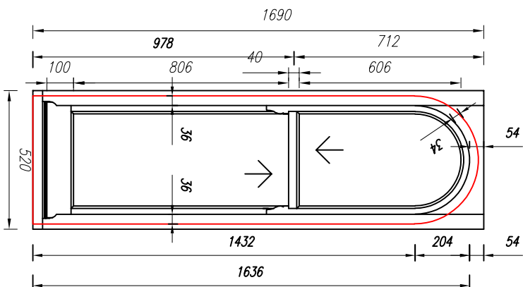
W4/W6 EXTERNAL VIEW - HORN TYPE BELSAY
