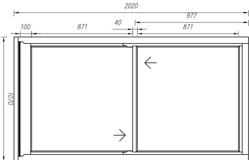
W2 EXTERNAL VIEW - HORN TYPE BELSAY
