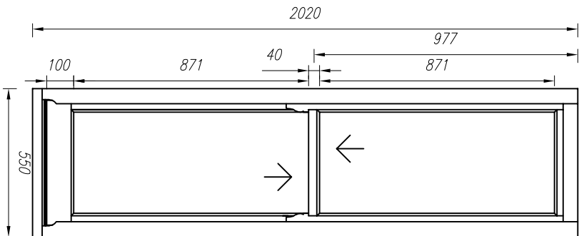
W1/W3 EXTERNAL VIEW - HORN TYPE BELSAY
