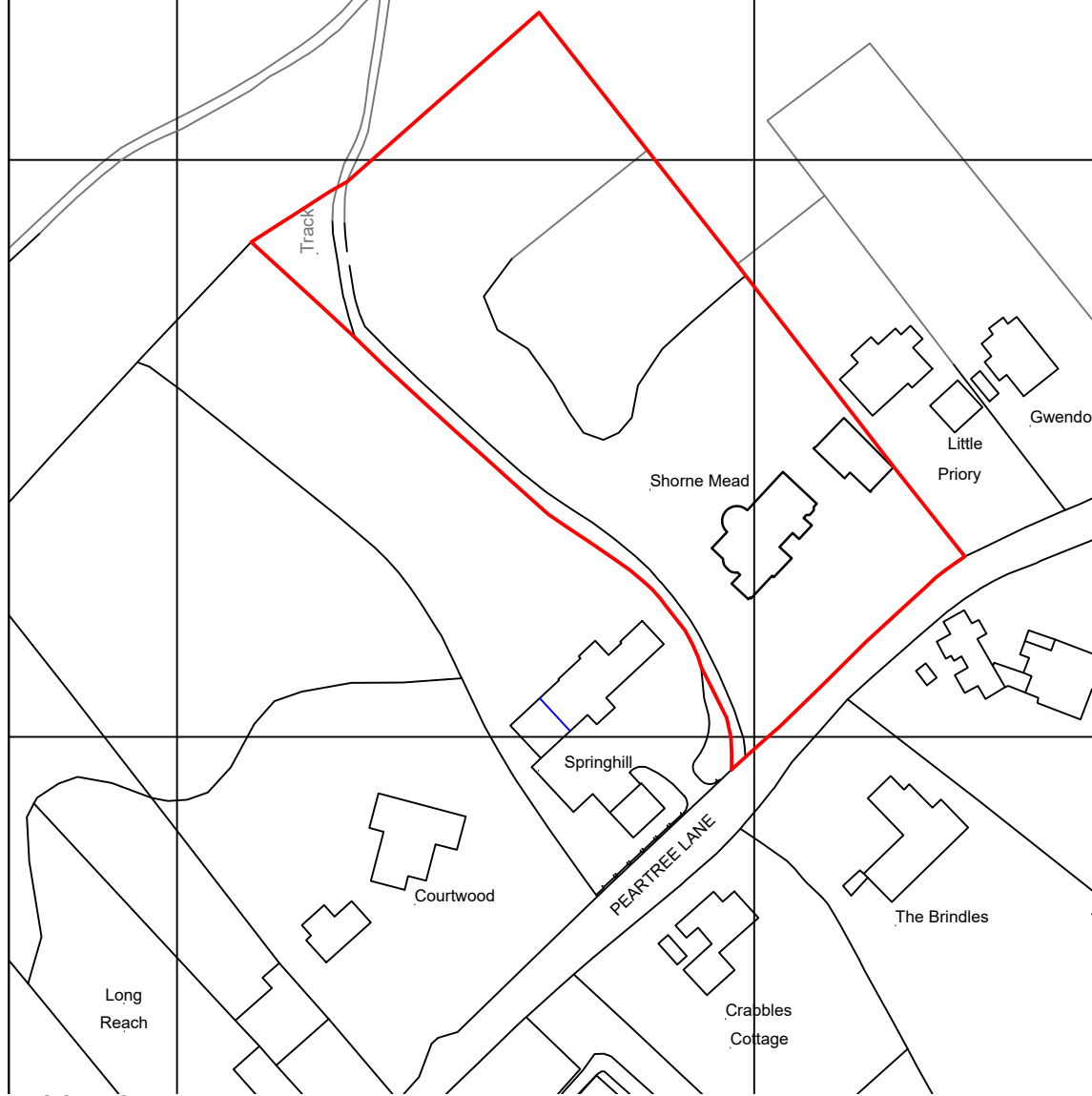
LOCATION PLAN 1:1250 Scale Bar at 1:1250
