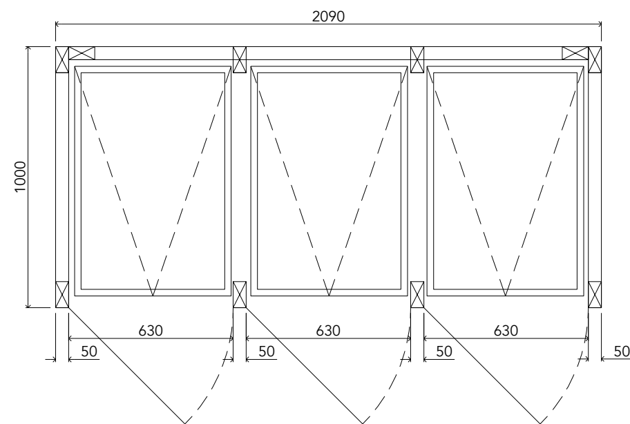
02 | 1:20 | INTERNAL LAYOUT
