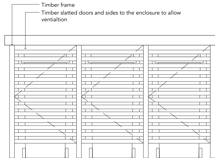
03 | 1:20 | FRONT ELEVATION
