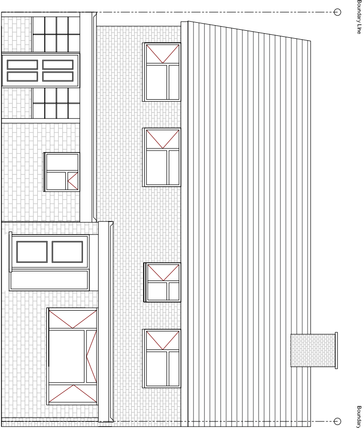
Pre Proposed Rear Elevation
