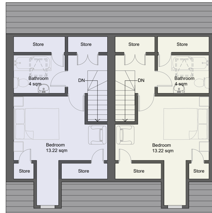
Proposed Loft Floor Plan
