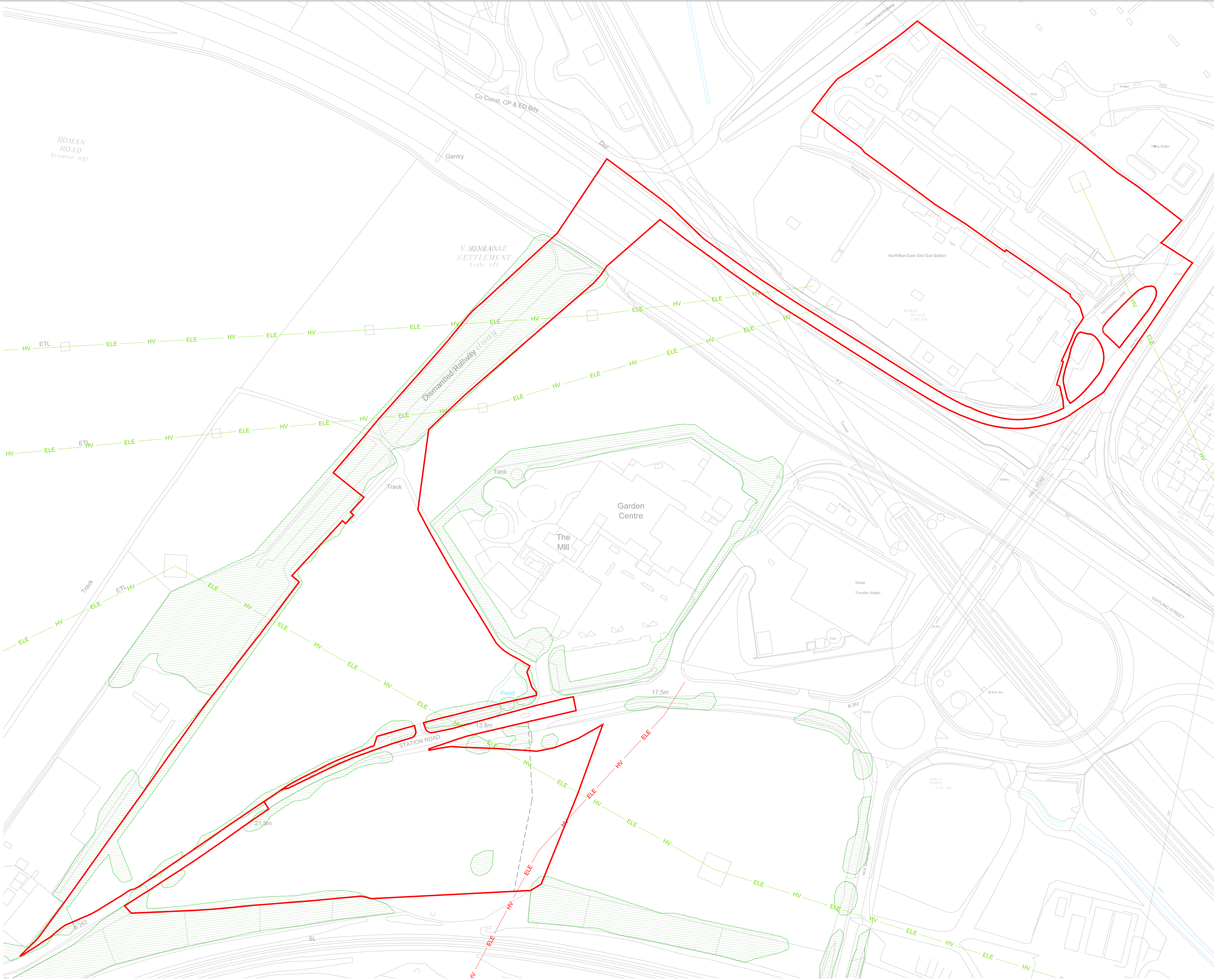
1 DARTFORD ENERGY HUB EXISTING SITE LAYOUT PLAN Scale: 1:1250@A1
