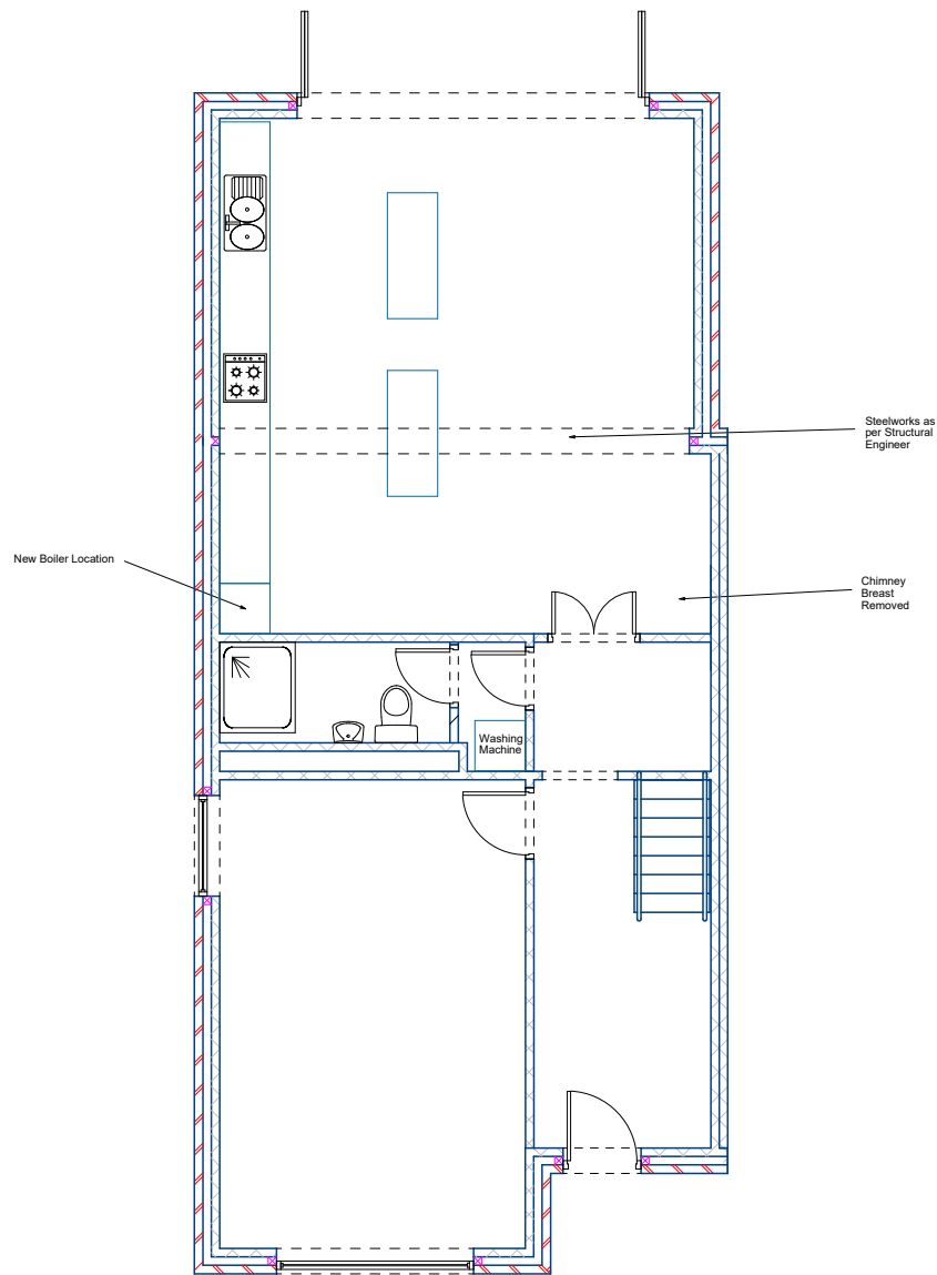
Proposed Layout
