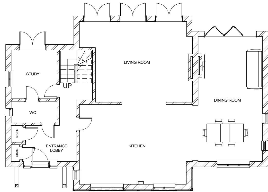
1 GROUND FLOOR 1 : 100
