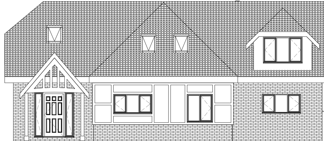
5 FRONT ELEVATION 1 : 100
