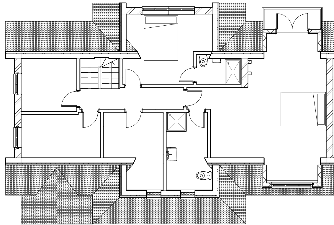
2 FIRST FLOOR 1 : 100
