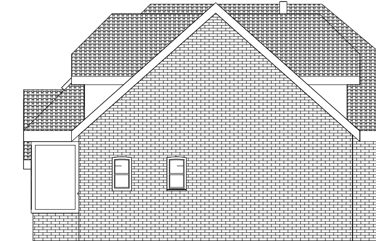
7 SOUTH SIDE ELEVATION 1 : 100
