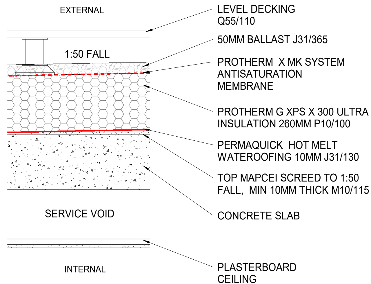
1 ROOF TYPE 1 (INVERTED HOTMELT ROOF)
