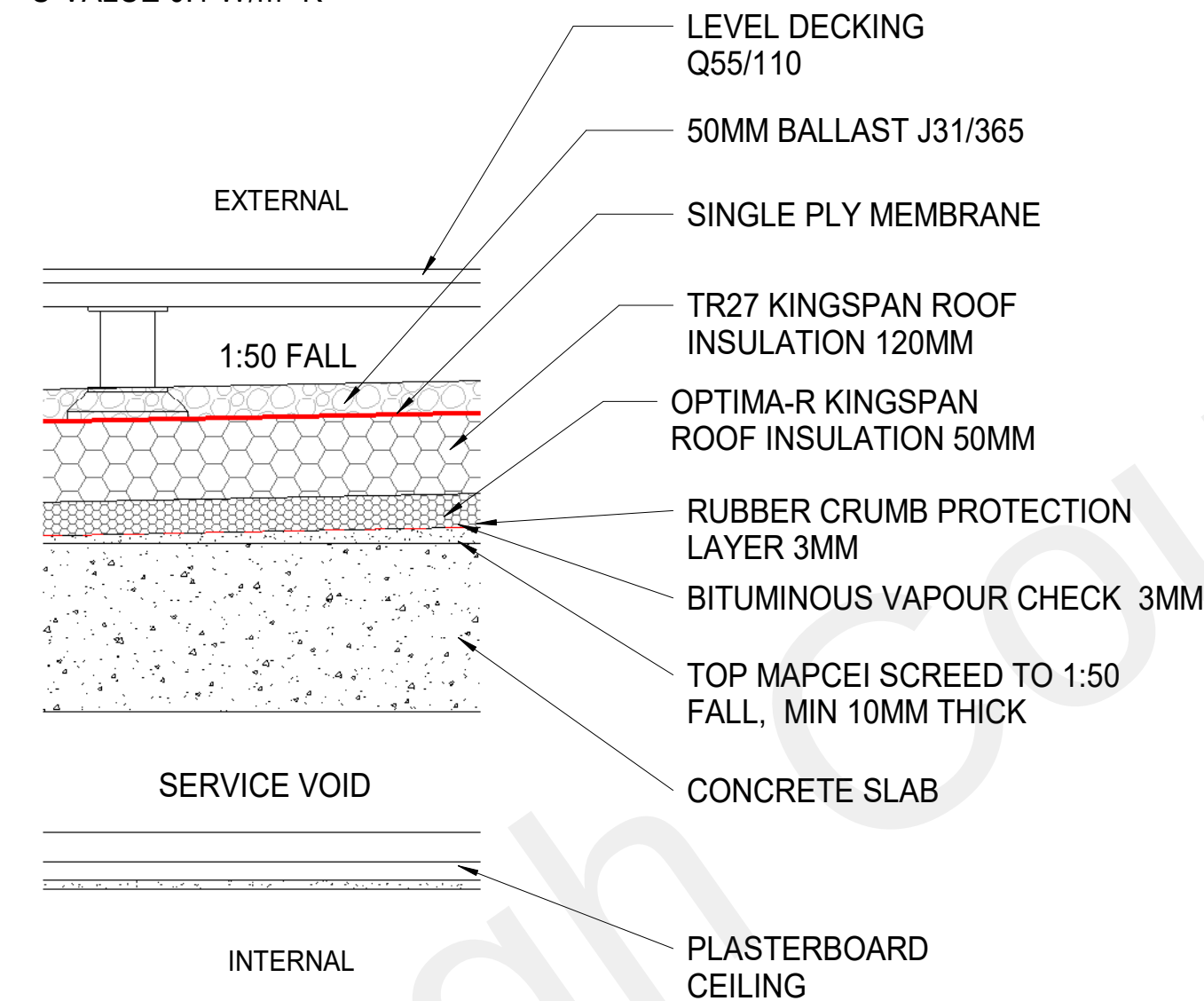
2 ROOF TYPE 2 (SINGLE PLY WITH OPTIM-R INSULATION)
