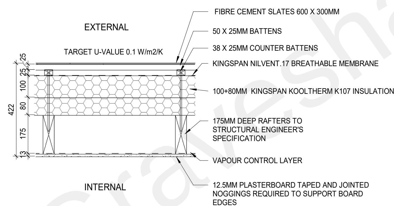
3 TYPICAL SLATE PITCHED ROOF DETAIL 1:10
