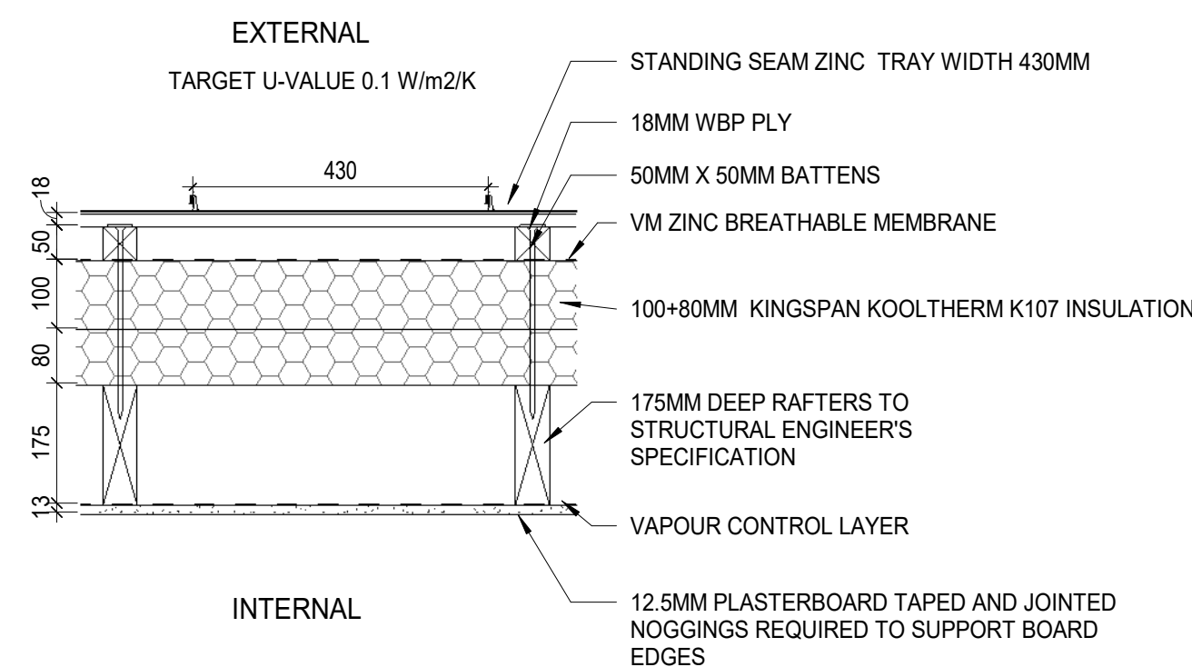
4 TYPICAL ZINC PITCHED ROOF DETAIL 1:10
