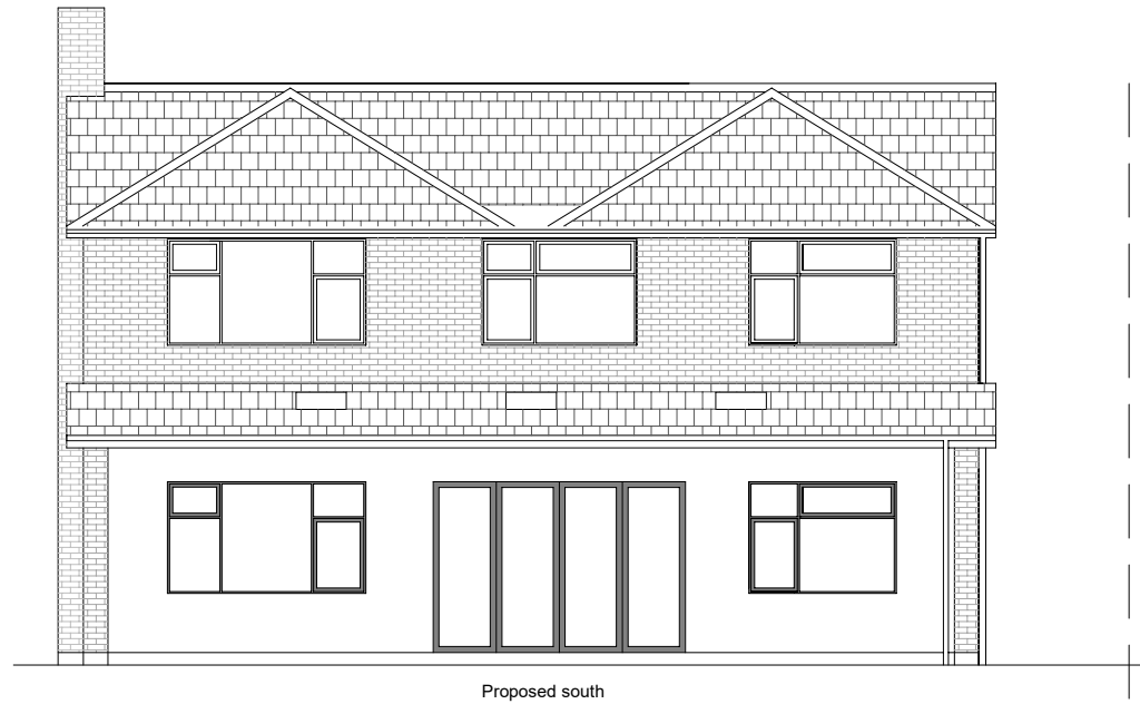
Proposed south
