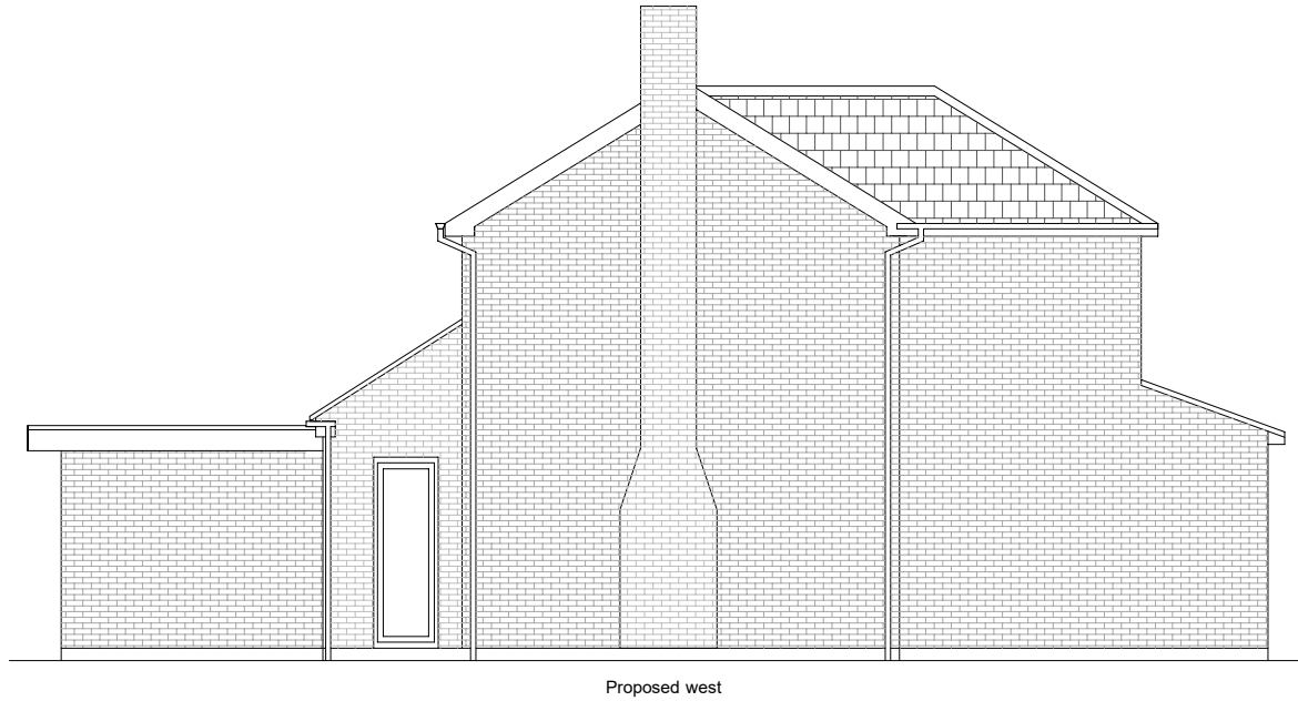
Proposed west
