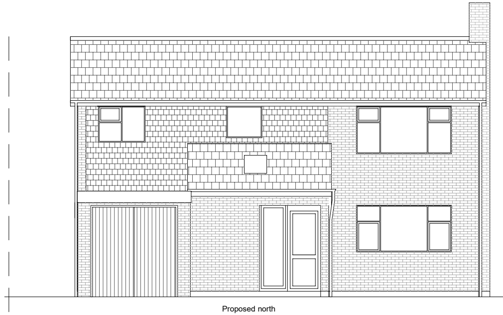
Proposed north
