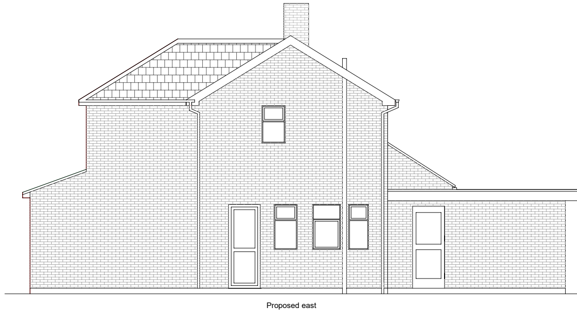
Proposed east
