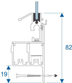
Section E
