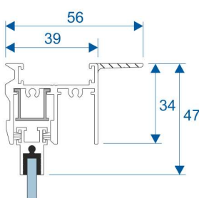
Section D
