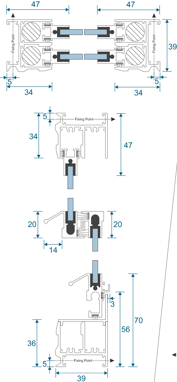
Face Fix
