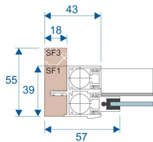
Section B
