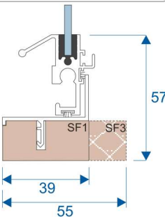
Section E
