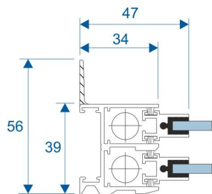
Section B
