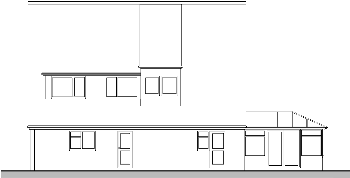
NORTH ELEVATION
