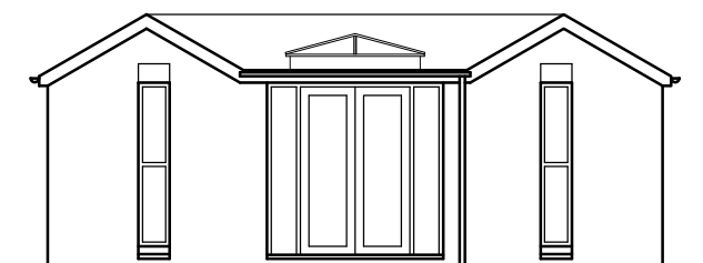
FRONT ELEVATION (1:100)
