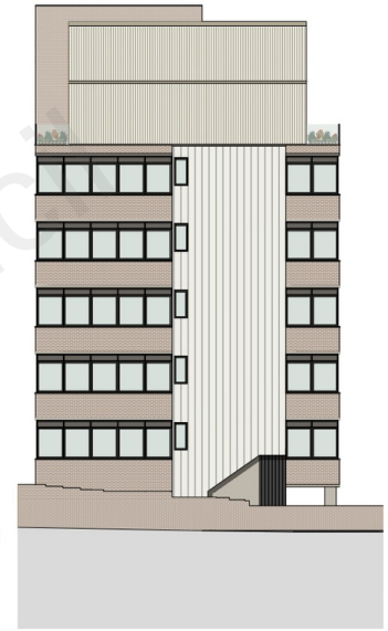
Proposed East Elevation
