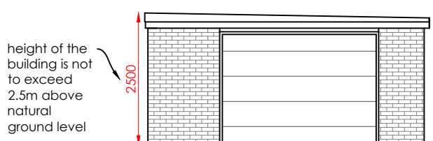
Rear elevation 1:100 0 2m 4m 6m 8m 10m 1:100 scale bar
