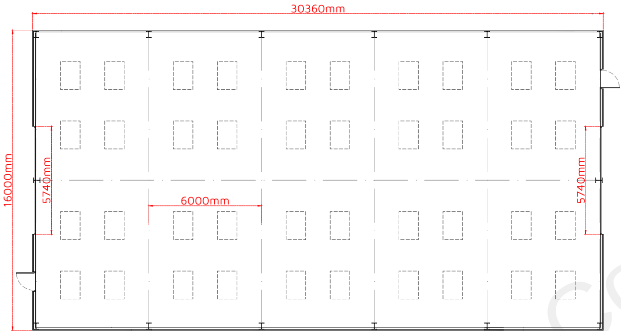
Proposed Ground Floor Plan 1:200 @ A3
