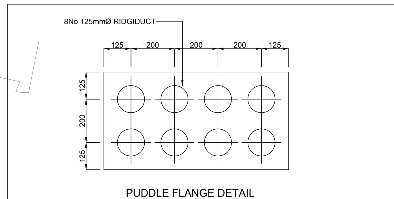
PUDDLE FLANGE DETAIL
