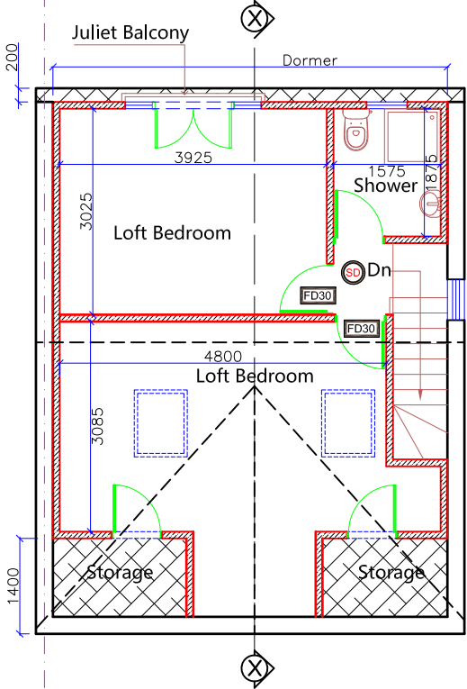
Proposed Loft Floor Plan
