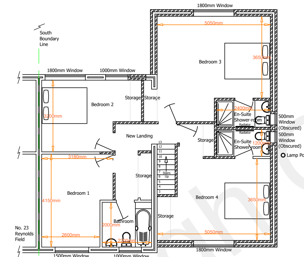
Proposed First Floor Plan "E" 1:100
