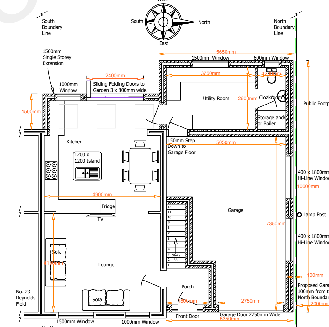
Proposed Ground Floor Plan "E" 1:100
