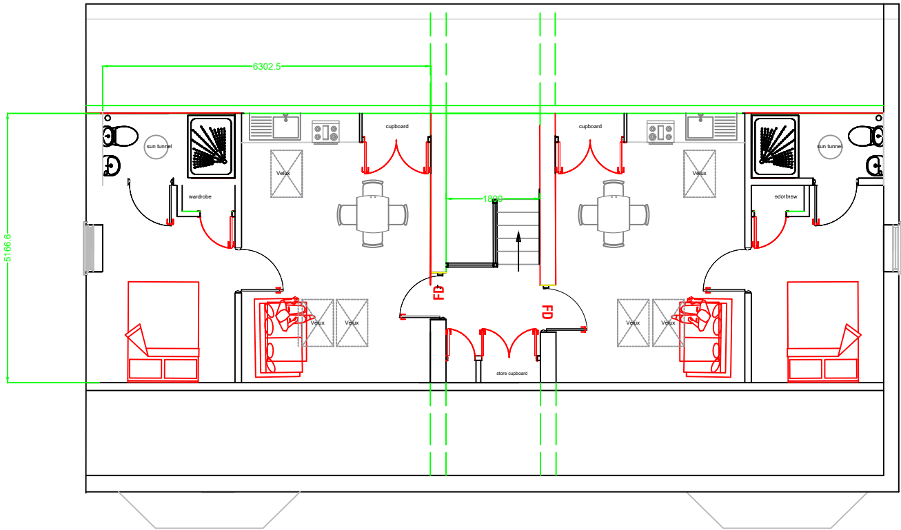
SECOND FLOOR
