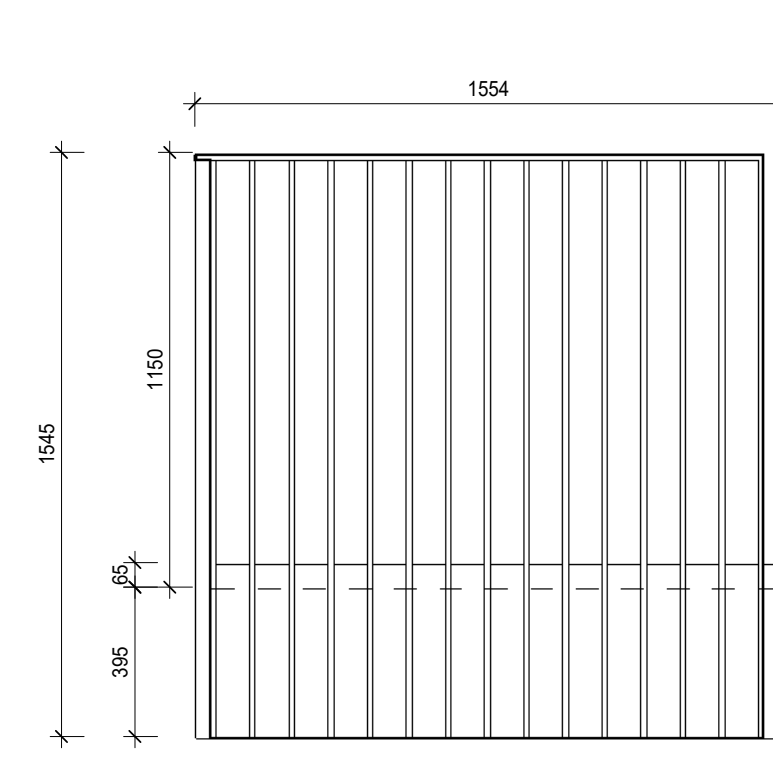
4 BALCONY TYPE 02 SIDE ELEVATION 02 1:20
