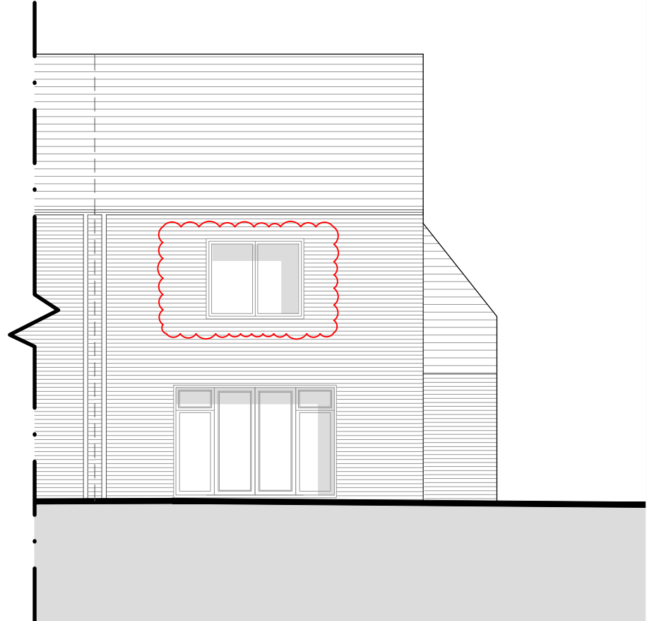
Rear Elevation @1:100
