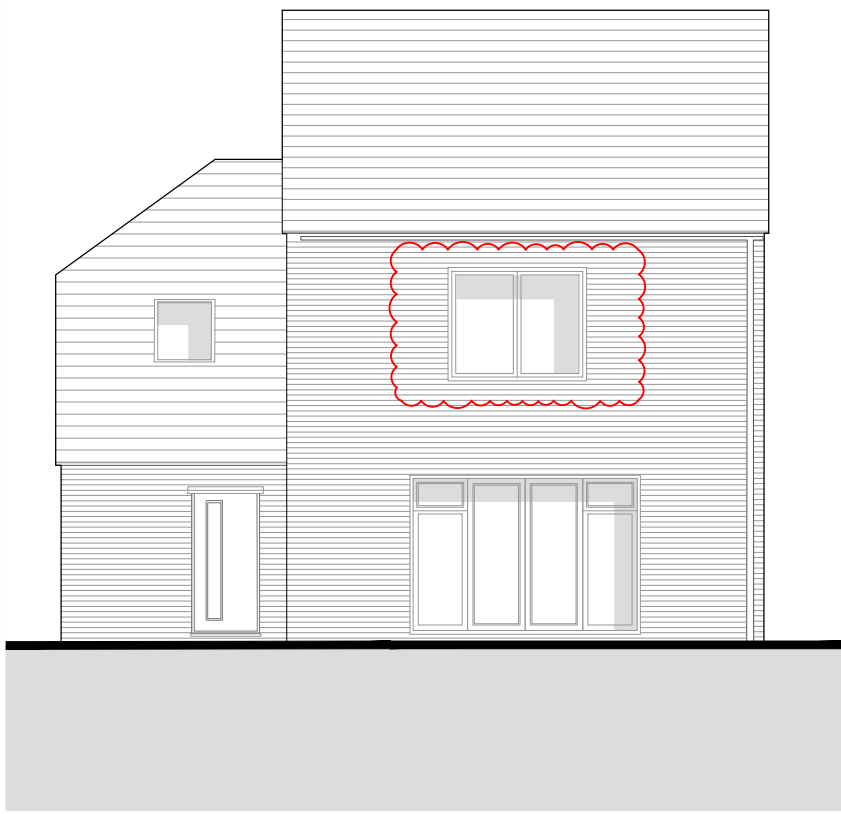
Rear Elevation @1:100
